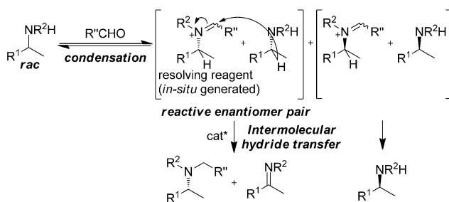
Scheme 1. Approaches for kinetic resolution of racemic amines.
