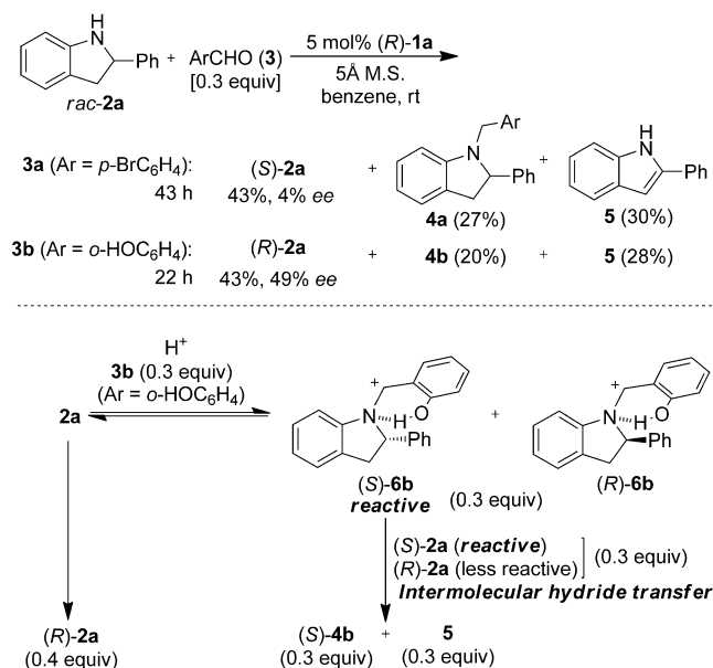
Scheme 2. First attempt at kinetic resolution of indoles and a proposed reaction mechanism.
